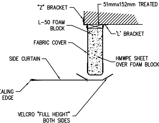
SIDE FRAME DETAILS
