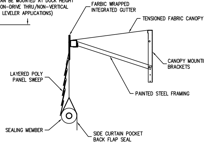
SEAL DETAILS
