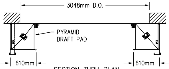
SECTION THRU PLAN
