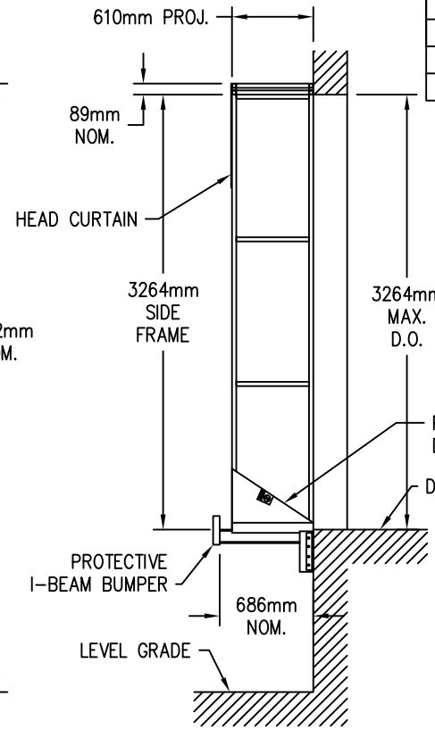
SECTION THRU ELEVATION
