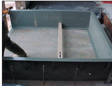
Set Dok-Box in place with squaring members - NO FORMS REQUIRED.
