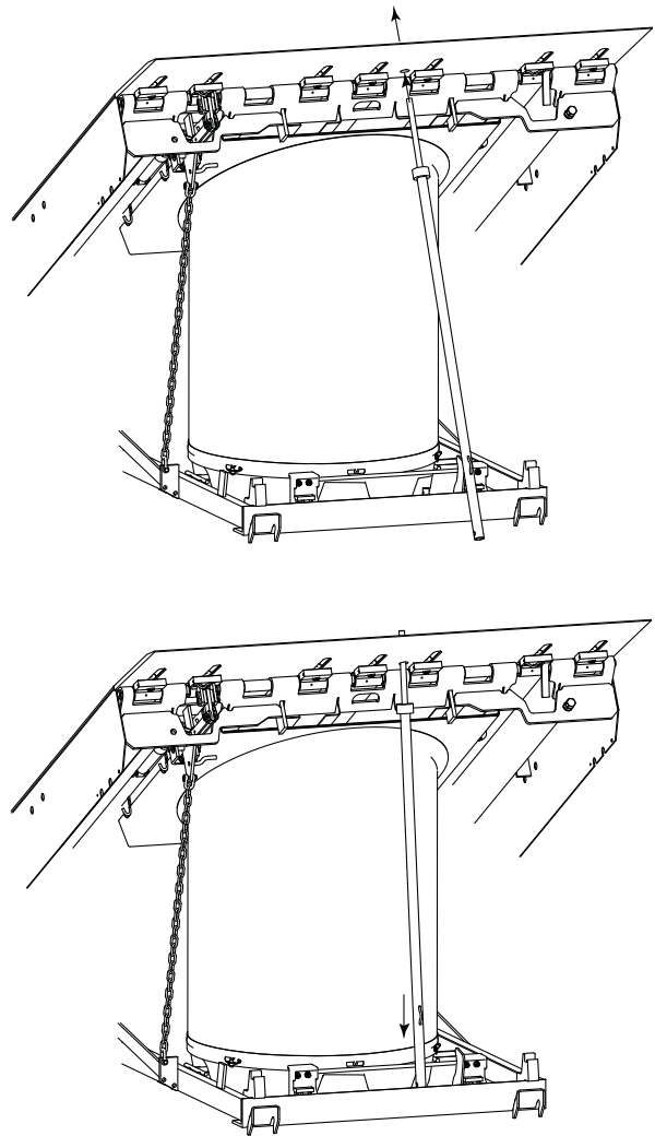
FIGURE 2 - INSTALL SAFE-T-STRUT™ SUPPORT
