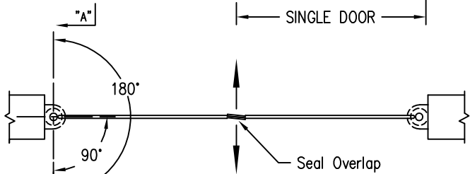
PLAN VIEW-DOUBLE ACTING DOORS
